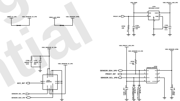
Proximity Detector
